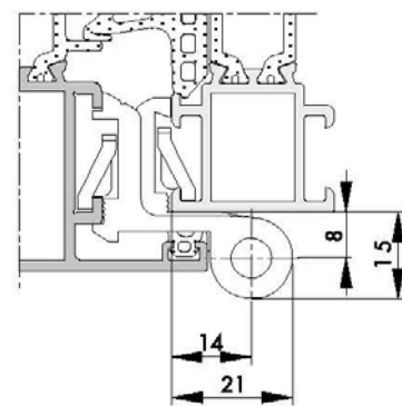
hardware installation space ALU D
