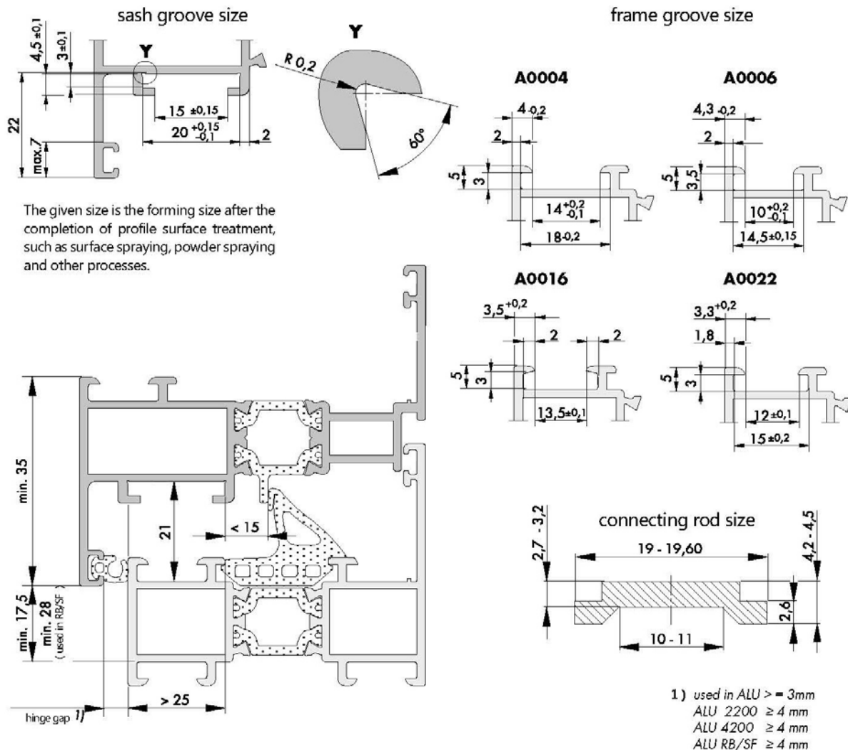
hardware installation space ALU 2200/ALU 4200
