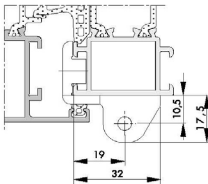
hardware installation space ALU RB/ALU SF
