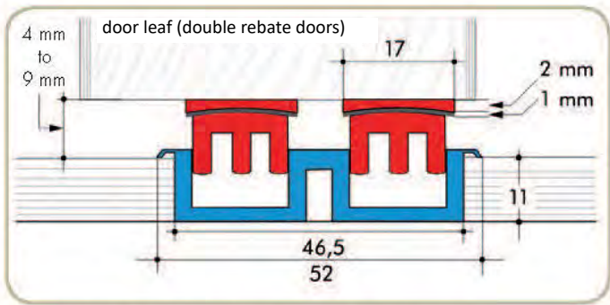
Model MFS 20 for double rebate doors Starting from approx. 9mm flooring / Magnetic force between upper and lower magnet profile (max. 5mm). Only available in silver anodized.
