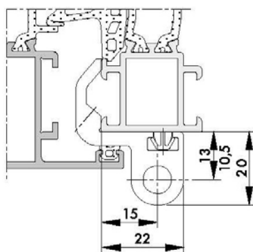
hardware installation space ALU 2200/ALU 4200
