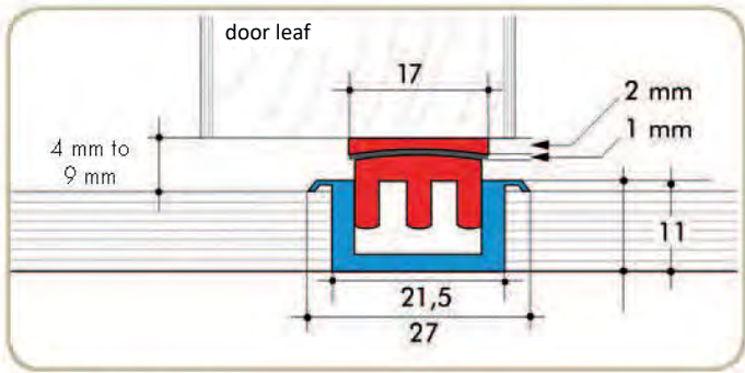
Model MFS 10 Starting from approx. 9mm flooring / Magnetic force between upper and lower magnet profile (max. 5mm)
