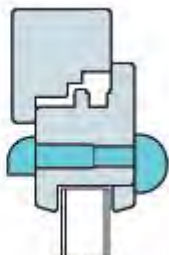
Installation in sash
