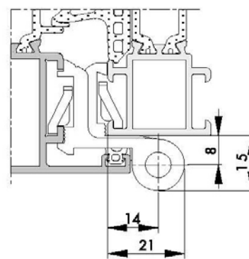
hardware installation space ALU D
