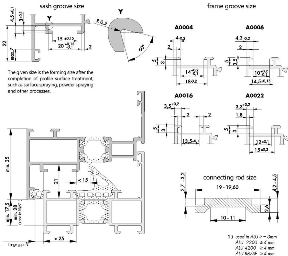
hardware installation space ALU 2200/ALU 4200
