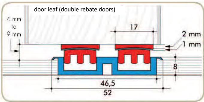
Model MFS 2 for double rebate doors Starting from approx. 6mm flooring / Magnetic force between upper and lower magnet profile (max. 5mm)
