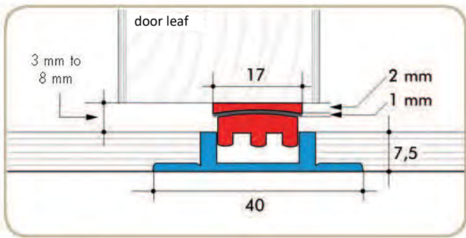
Model MF 1 Starting from approx. 6mm flooring / Magnetic force between upper and lower magnet profile (max. 5mm)
