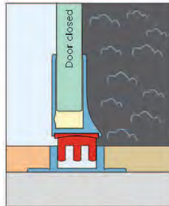
Door closed Magnet goes up and provides perfect sealing
