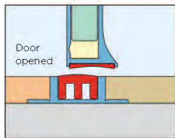
Door opened Magnet stays down, the pass is absolutely barrier-free
