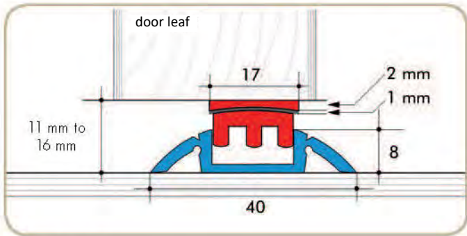
Model MA 1 On the floor / Magnetic force between upper and lower magnet profile (max. 5mm)
