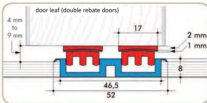
Model MFS 2 for double rebate doors
